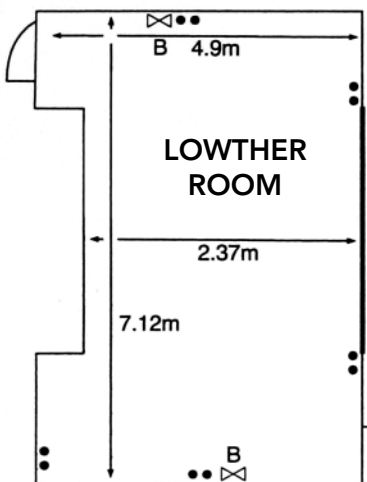
Height 3.35m Ground Floor
